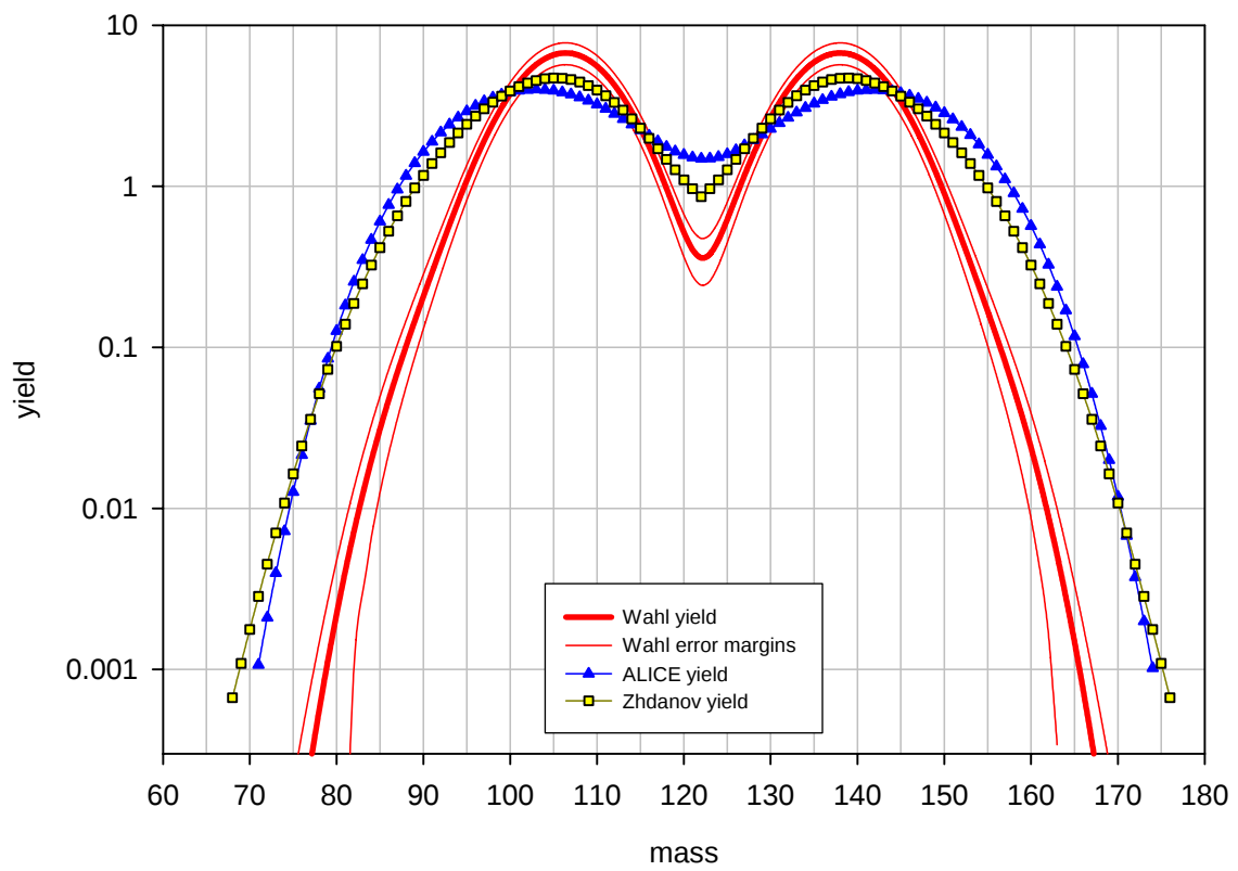
Benchmark B: ^{244}\text{Cm} at 13 MeV, pre-neutron emission mass distribution
